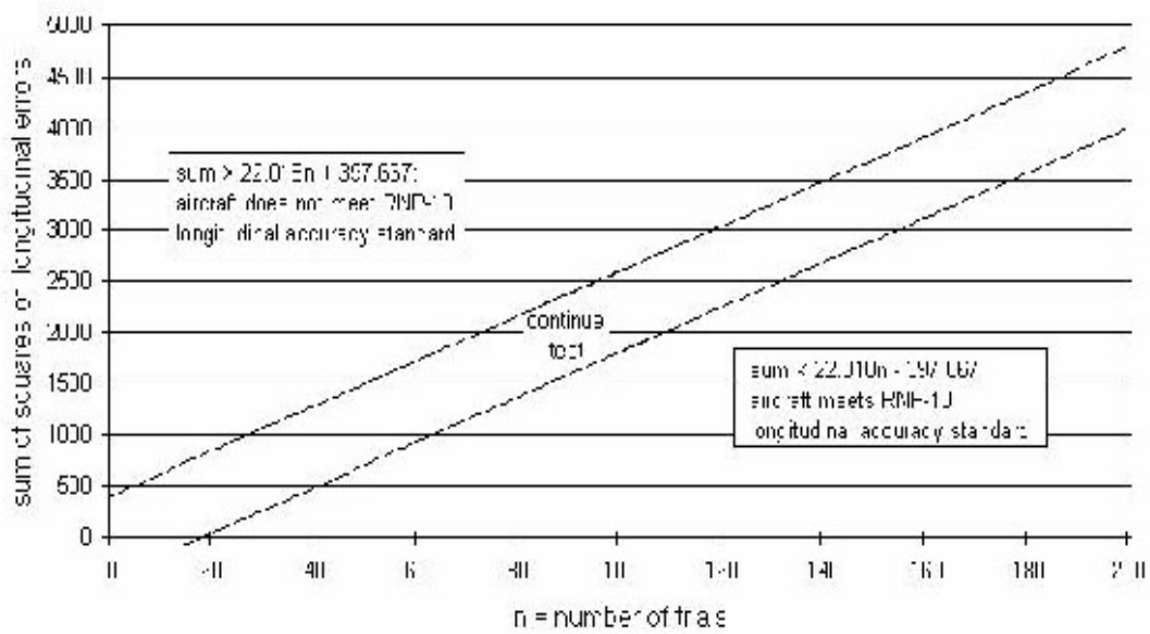
Figure 2: Acceptance, Rejection and Continuation Regions for Sequential Test of Longitudinal Accuracy
