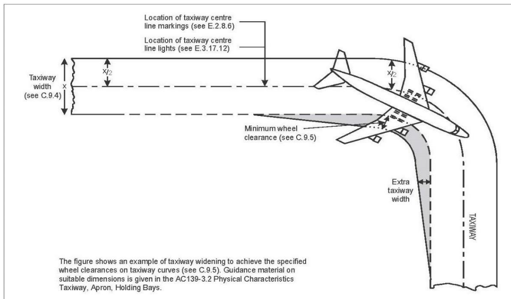
Figure C-2. Taxiway curve
