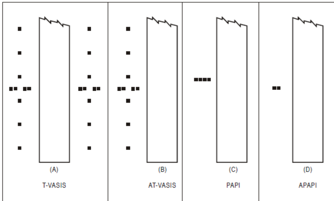
Figure E-16. Visual approach slope indicator systems
