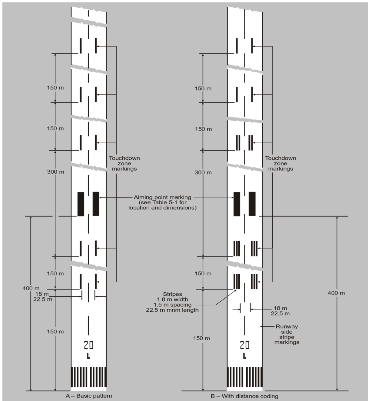
Figure E-5. Aiming point and touchdown zone markings
